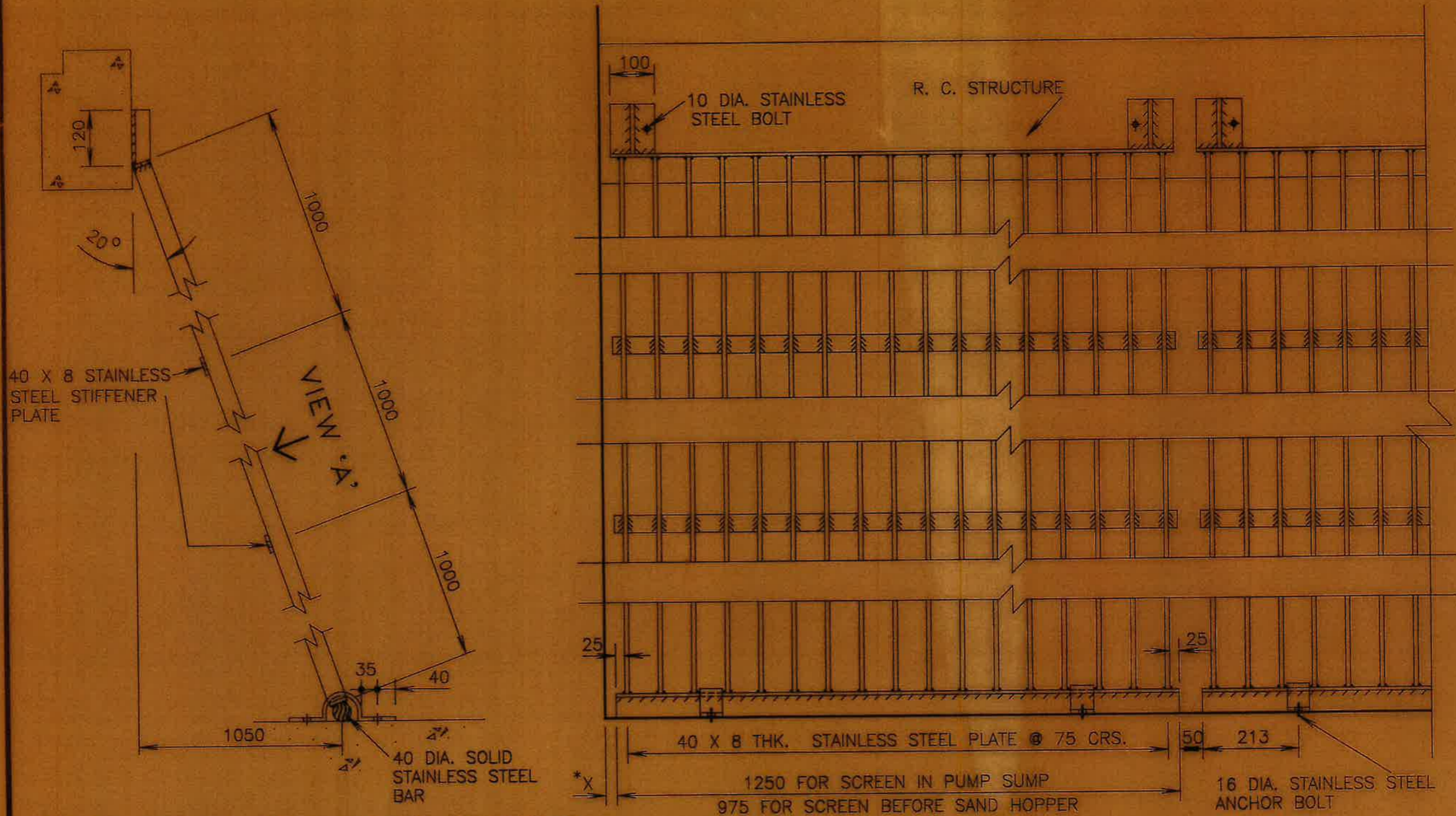
PUMP SUMP AND SAND HOPPER SCREEN DETAILS SCALE : 1 : 10
