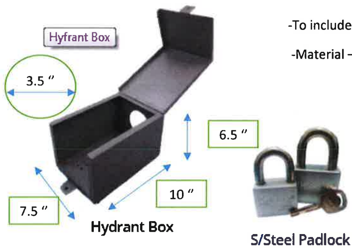
Figure 4. Hydrant Box come with padlock
